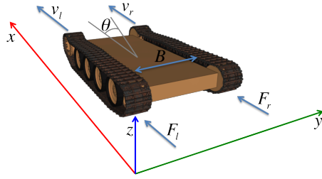
Figure 4: LandShark unmanned ground vehicle; (a) The vehicle; (b) Coordinate system and variables used to derive the model; (c) Control system diagram used for cruise control.
