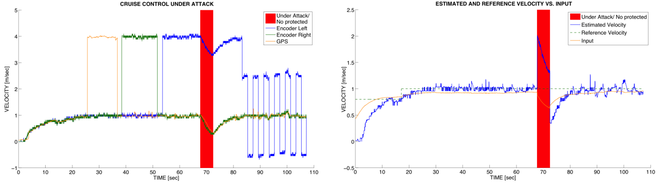
Figure 6: Experimental results; (a) Comparison of velocity estimated from the encoders’ and GPS measurements; (b) Reference speed, the estimated speed, and the input applied to the motors.
