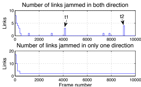
Figure 16: Number of links jammed in 2/1 direction used for communication
