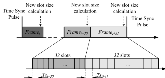
Figure 10: Slot size randomization on a frame-by-frame basis
